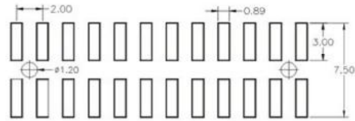
PCB LAYOUT
