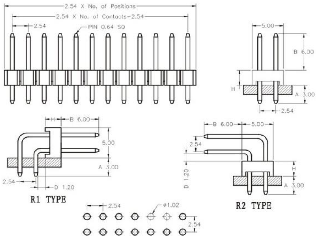
PCB LAYOUT
