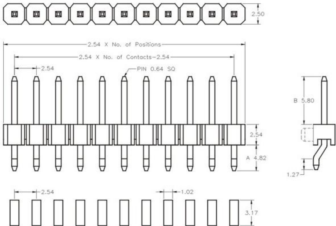
PCB LAYOUT
