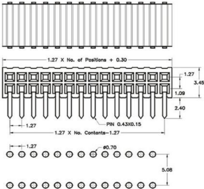
PCB LAYOUT
