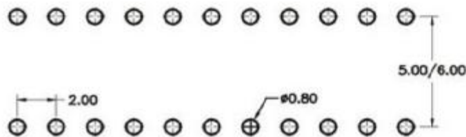
PCB LAYOUT
