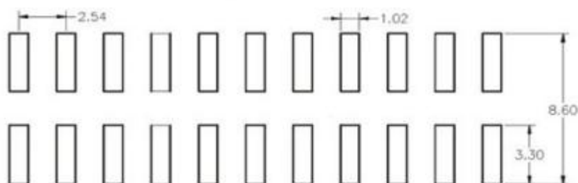
PCB LAYOUT
