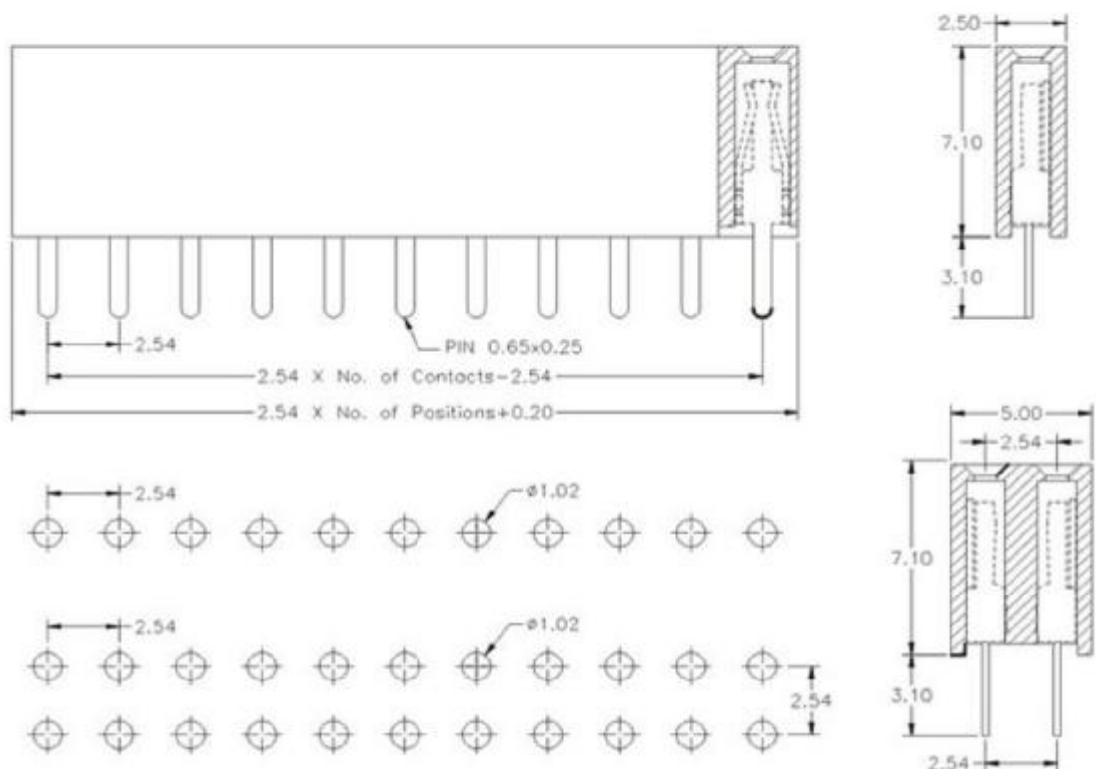
PCB LAYOUT
