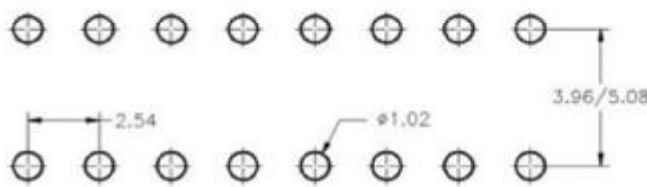
PCB LAYOUT
