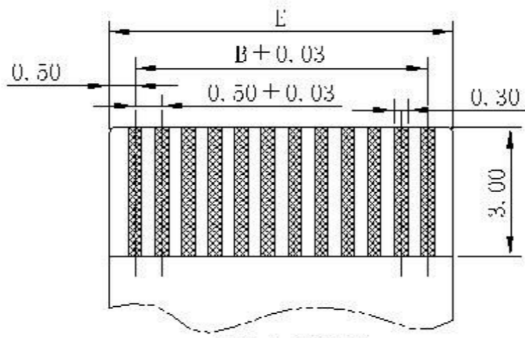
FPC LAYOUT (THICKNESS: 0.3 ± 0.03)
