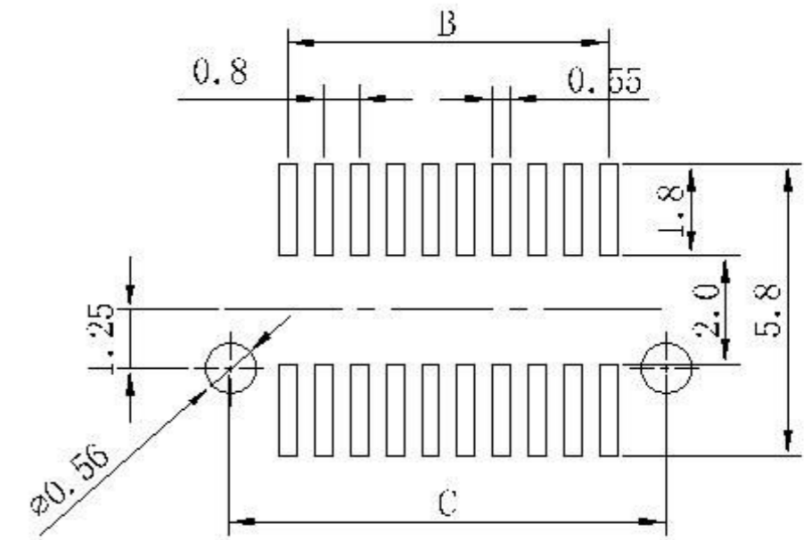
PCB Layout for Surface Mounting
